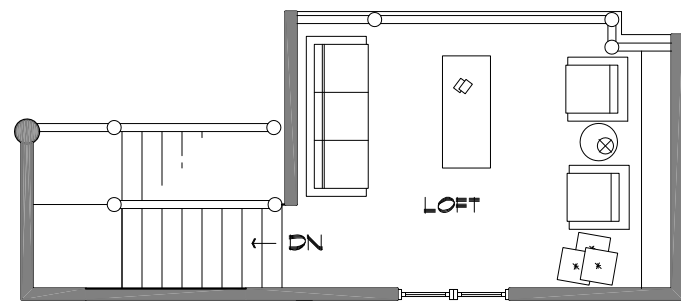
○ LOFT FLOOR PLAN SCALE 1/8" = 1'-0" AREA: 190 SQ. FT.
