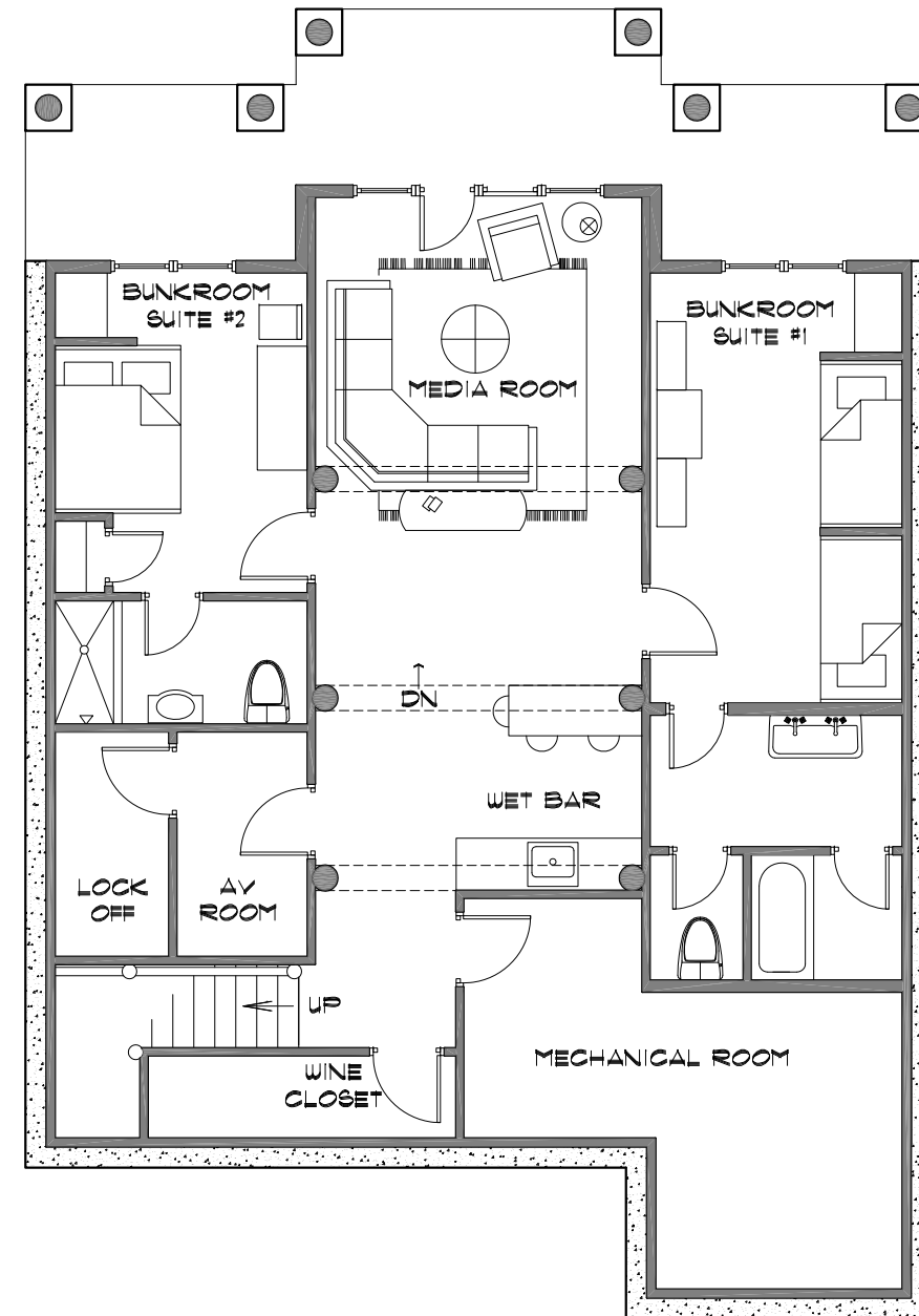
○ LOWER LEVEL FLOOR PLAN SCALE 1/8" = 1'-0" AREA: 1412 SQ. FT.
